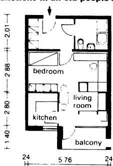
③ One-person apartment 41 m 2
